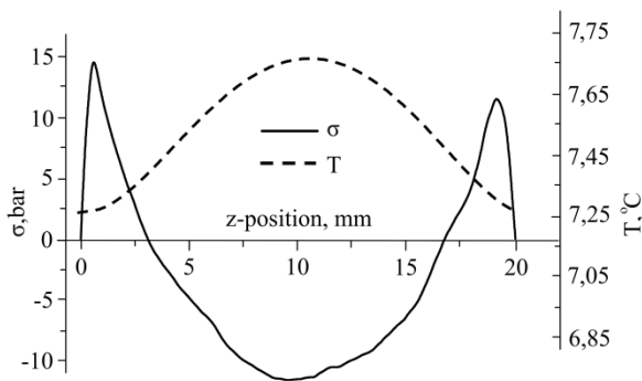
Fig. 5. The distribution of T(z) , obtained by double integration of the function \sigma(z) at y=10 mm
