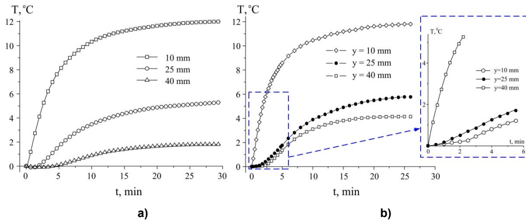
Fig. 6. The distributions of T(t) in three points of y -position, obtained by measuring the y - x -surface (a) and by double integration of \sigma(t) function shown in fig. 3 (b)
