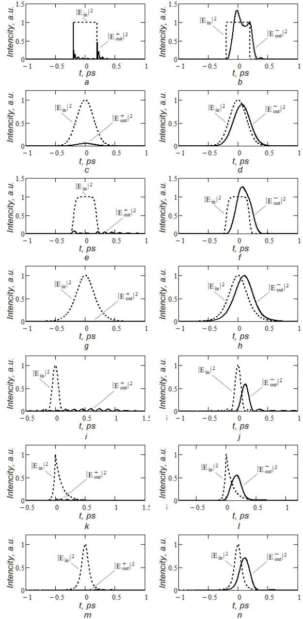
Fig. 2. Pulse intensity envelopes as a result of scattering: (a), (b) - of rectangular pulse 0,4 ps; (c), (d) - Gaussian ( \sigma=0,2 ps; C=0,5 ); (e), (f) - super-Gaussian ( \sigma=0,2 ps; m=4 ); (g), (h) - soliton-like ( \sigma=0,2 ps); (i), (j) - ultra-short sinc - pulse ( \sigma=2 ps; N_i=50 ); (k), (l) - exponential ( \sigma_1=0,05 ps; \sigma_2=0,2 ps); (m), (n) - Lorentzian ( \sigma=0,1 ps)
